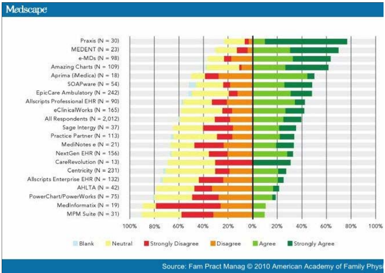
Response Spectrum: 'Our EHR Vendor Provides Excellent Training and Support'
